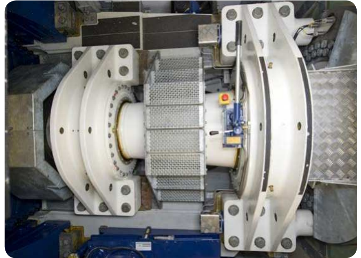
SKF self-aligning bearing system, with a locating spherical roller bearing on the left hand side, and a non-locating CARB toroidal roller bearing on the right hand side.
